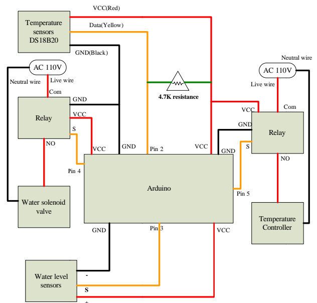
Fig.3 Hardware wiring diagram
