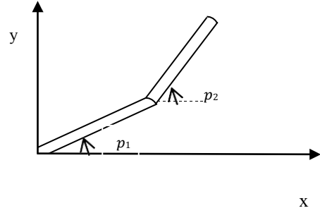
Fig. 2: Generalized coordinates for planar elbow manipulator with remotely driven links
