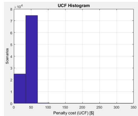
Figure 5. Uncertainty cost function for different powers at 50 MW wind speed.
