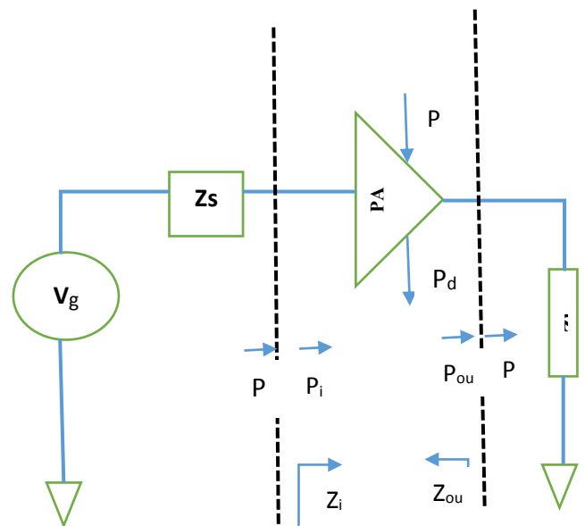
Figure 1: Power Amplifier
