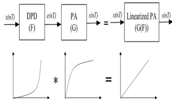
Figure 6: Predistortion Technique
