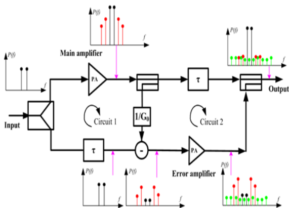
Figure 4: Feedforward Technique
