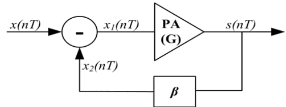
Figure 5: Feedback Technique
