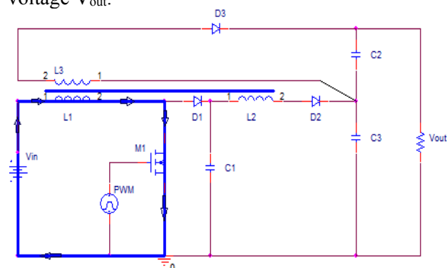
Fig. 2. Mode 1 operation
