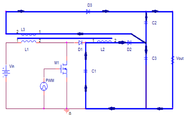
Fig.4. Mode 3 operation
