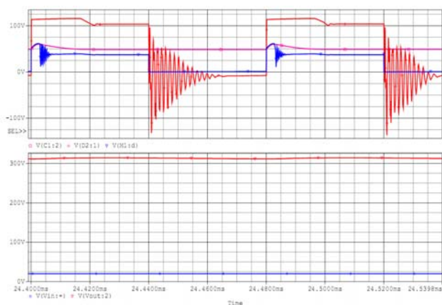
Figure 7. Simulated input and output voltage, voltage stress rectifier of the diodes D2 of the converter. For this simulation, the transformation ratio is fixed at a standard value duty ratio = 0,5, k=0.95
