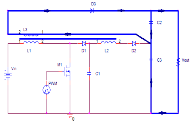
Fig. 5. Mode 4 operation
