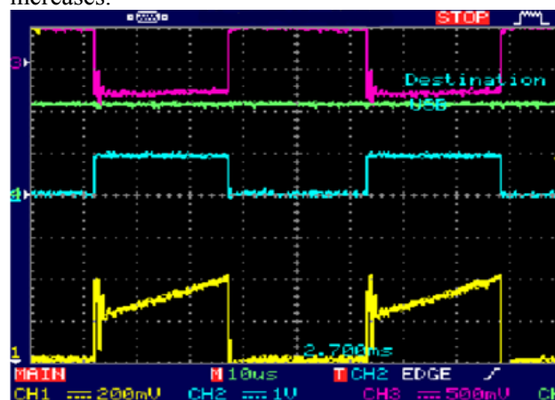
Fig. 9. The waveforms: Current of the MOSFET (line yellow); Pulse wide modifier driver (line blue);
