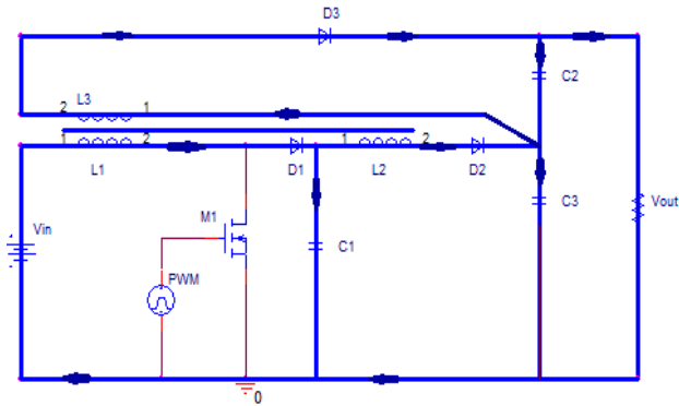
Fig. 3. Operation of converter at the mode 2
