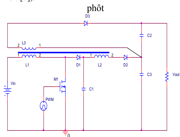
Fig. 1. Diagram Boost-Flyback coupled magnetic of a converter with stage RS
