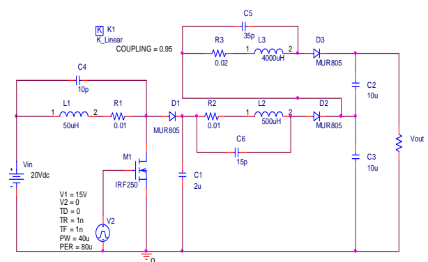
Fig. 6. Simulation Boost-Flyback coupling magnetic-recovery stage
