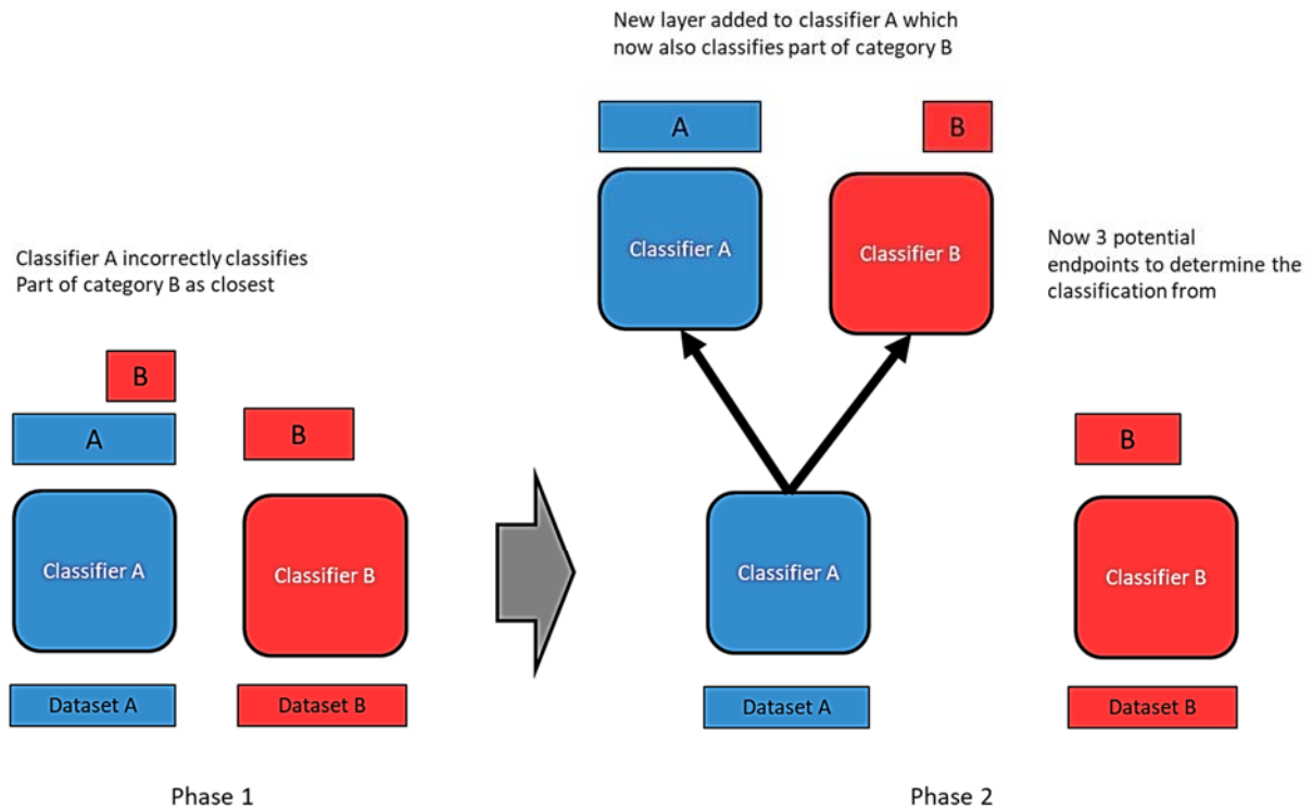
Figure 1. Schematic of the classifier in action. Phase 1 realises that classifier A also classifies part of category B better. Phase 2 then adds a new layer to layer 1 of classifier A, to correctly re-classify this problem.
