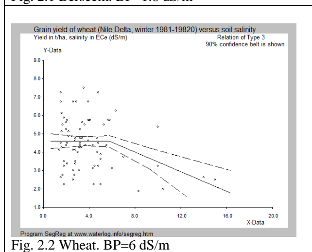
Fig. 2. Examples of results using the MH model for two Egyptian crops
