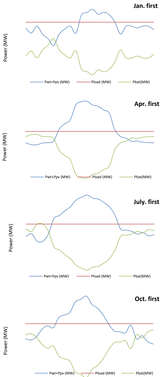
Fig.5 - The simulation results of hybrid system for four days.
