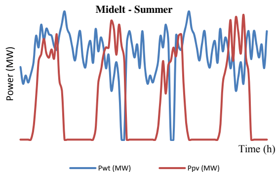
Fig.6 - The simulation of WT and PV in Midelt.
