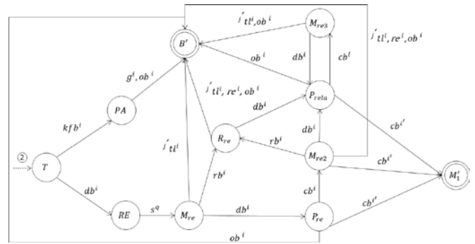
Fig. 1 (b) FSM for a touchdown
