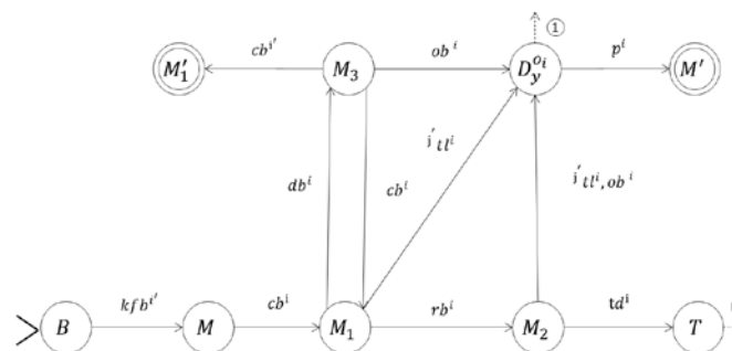
Fig. 1 (a) FSM for the game start
