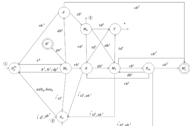
Fig. 1 (c) FSM to describe plays in the field
