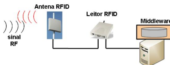
Fig.6: RFID Architecture
