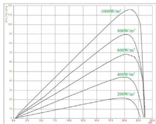
Fig. 6 P-V curve for parallel configuration
