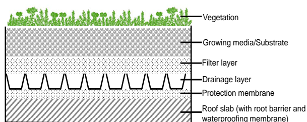
Figure 1 – Green roof experimental set up and schematic representation [12]
