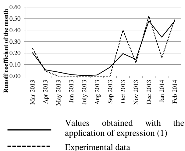
Figure 2 – Monthly runoff coefficient of the pilot GR system.
