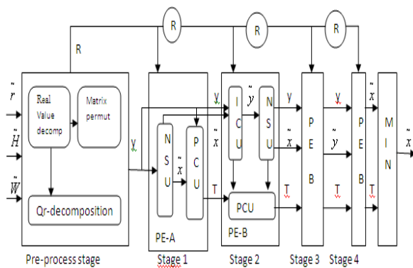
Fig.2 VLSI architecture of MIMO signal detector
