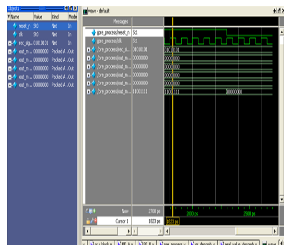
Fig.3 Output Waveform of Pre-processing block
