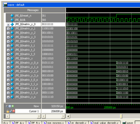
Fig.5 Output Waveform of PE-B
