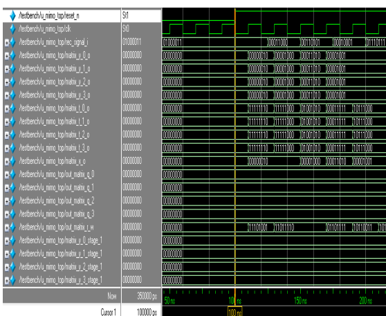
Fig.6 Output Waveform of MIMO detector
