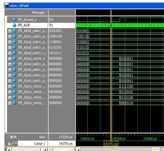
Fig.4 Output Waveform of PE_A
