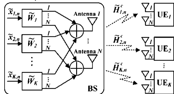
Fig 1: LTE-A downlink transmission system
