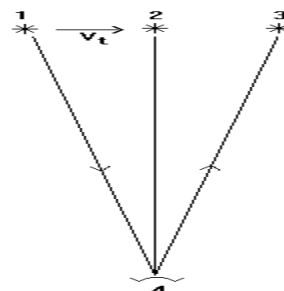
Fig.11. Scheme of Kozyrev telescope. 1 – focusing mirror, 2 - slot, 3 - detector, 4 – light-proof lid.
