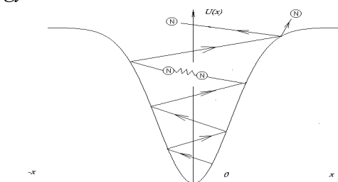
Fig.13. Oscillation of Nitrogen molecule in potential well of catalyst.
