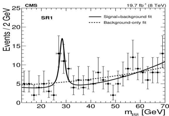
Fig.8. Peak of energy at 28GeV
