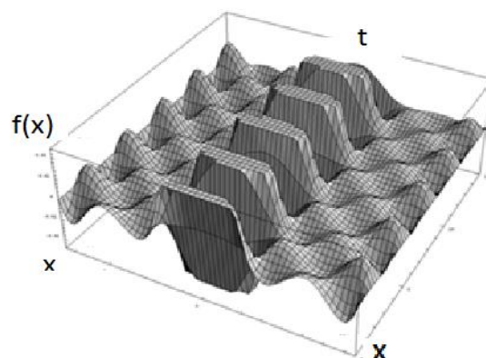
Fig.3. During the motion, the packet f(x) will appear and disappear periodically.
