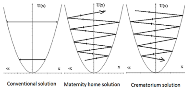
Fig. 10. Solution of UQT for harmonic oscillator
