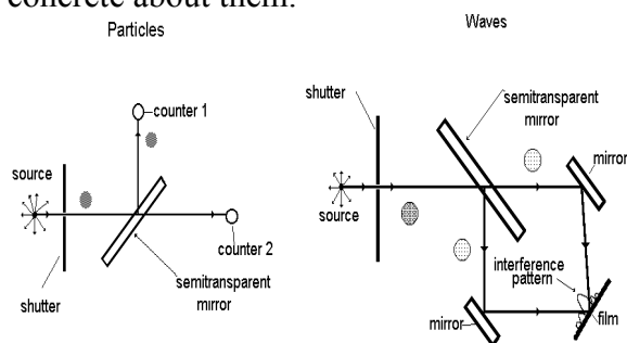
Fig.1. Experiments with individual photons on semitransparent mirror
