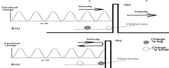
Fig.14. Illustration of the tunnel effect
