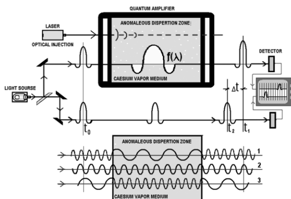
Fig.7. Experiments of L. Wang superluminal light propagation.
