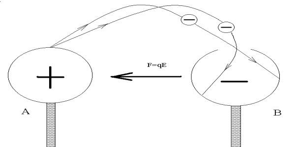
Fig. 9. Work for transferring the charge depends on the mode of transferring and on the path.
