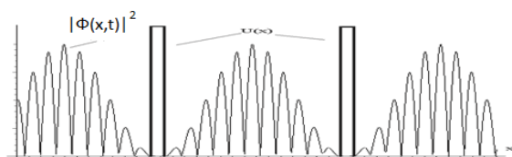
Fig.15. Visual image of particles passing through two potential barriers - scheme of New Maxwell Demon.
