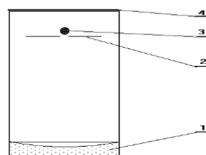
Fig.11. Scheme of Kozyrev telescope. 1 – focusing mirror, 2 - slot, 3 - detector, 4 – light-proof lid.
