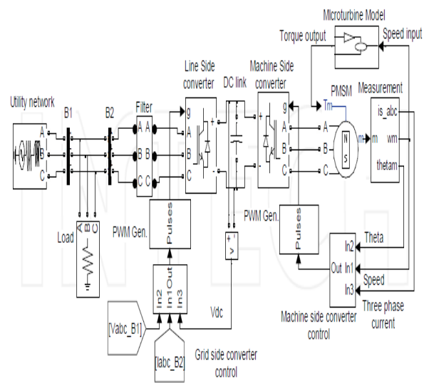
Fig. 5. Matlab/ Sim Power Systems implementation of MTG system connected to grid
