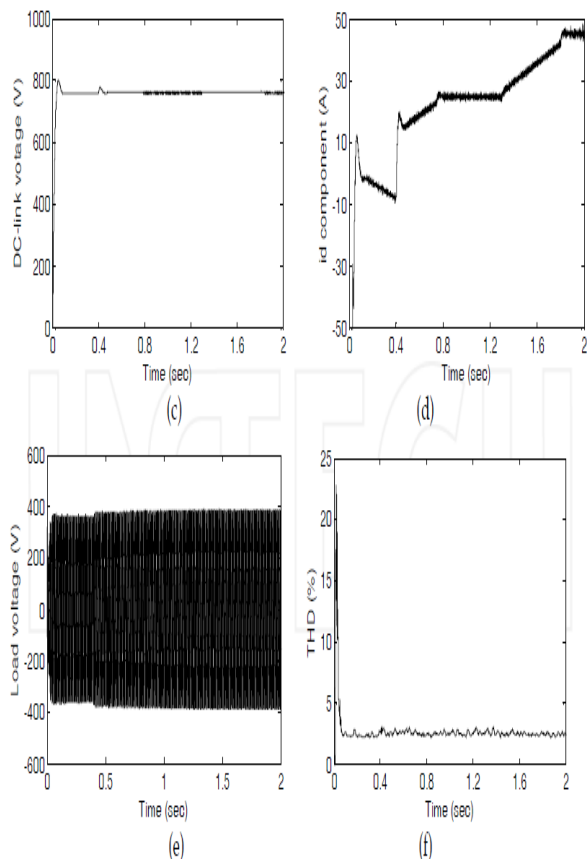
Fig. 7. (a) Electromagnetic torque variations of the PMSM (b) Detailed variations of the stator current of PMSM (c) DC link voltage variation (d) i_d component of the injected grid current (e) Line to line voltage at the load terminals (f) %THD variation at the load terminals.
