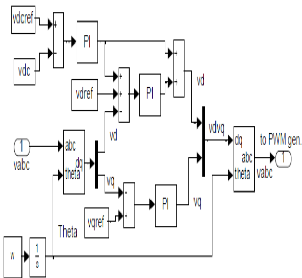
Fig. 4. Control structure for islanding mode operation
