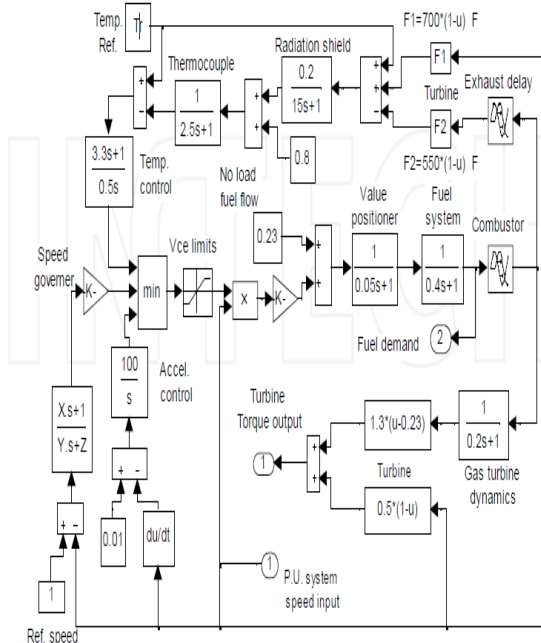
Fig. 2. Simulink model of the microturbine
