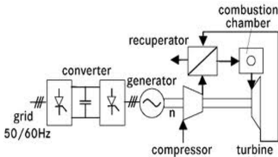
Fig.1. Microturbine generator system (MTGS)
