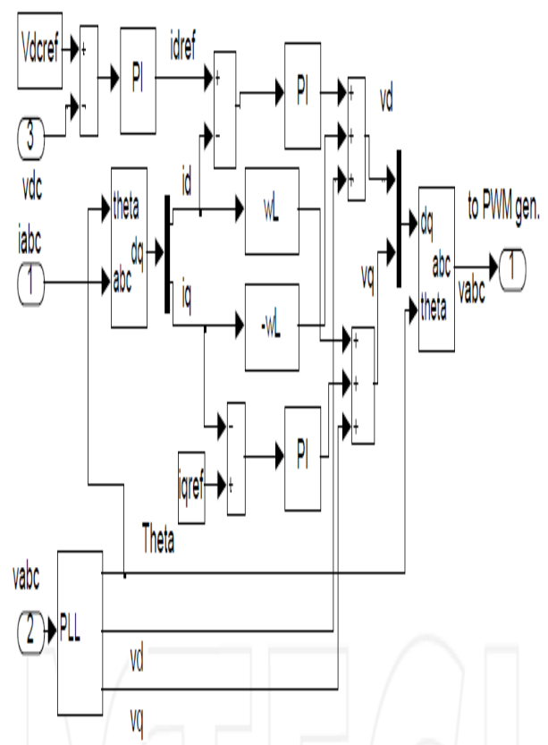
Fig.3. Grid side converter controller
