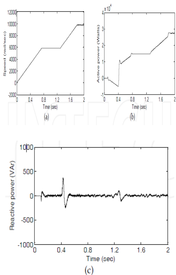
Fig. 6. Motoring and generating operation of PMSM (a) speed variation of PMSM (b) active power variation at the grid side of the MTG system (c) reactive power variations at the grid side of the MTG system
